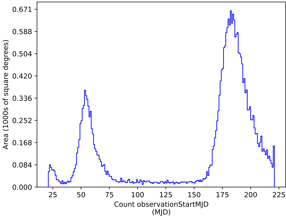
too_5_4v3.4_10yrs r: Count observationStartMJD
