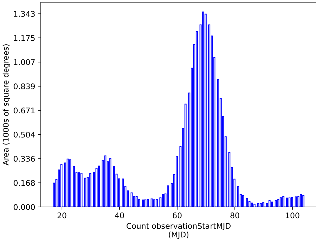
too_5_4v3.4_10yrs g: Count observationStartMJD
