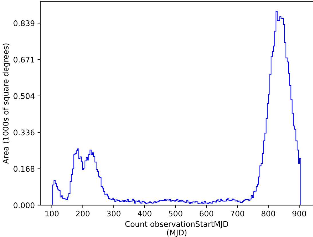
too_5_4v3.4_10yrs : Count observationStartMJD
