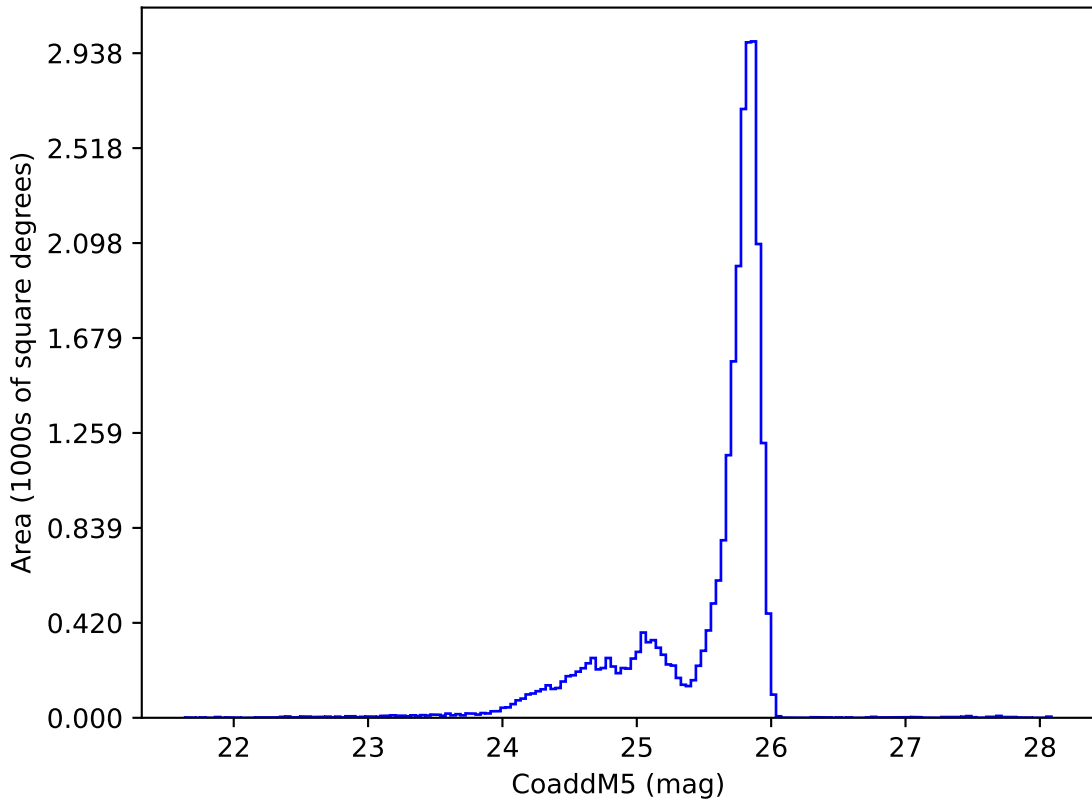
too_5_4v3.4_10yrs z: CoaddM5
