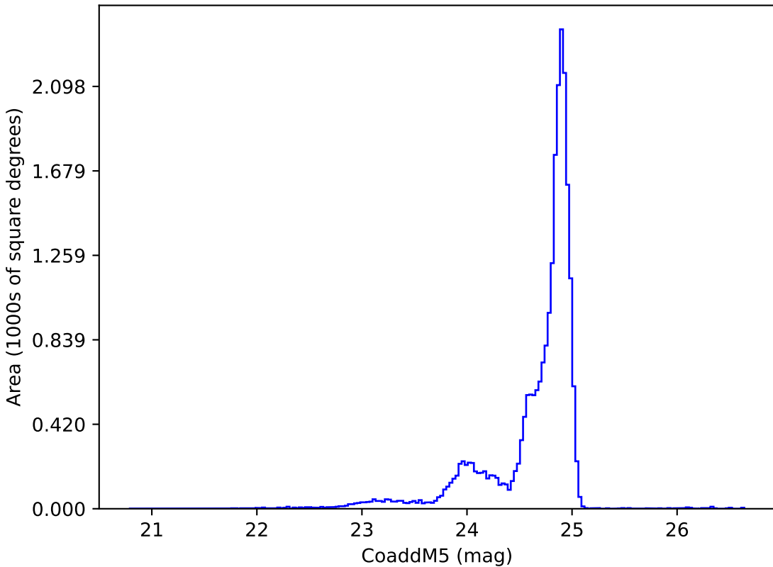
too_5_4v3.4_10yrs y: CoaddM5
