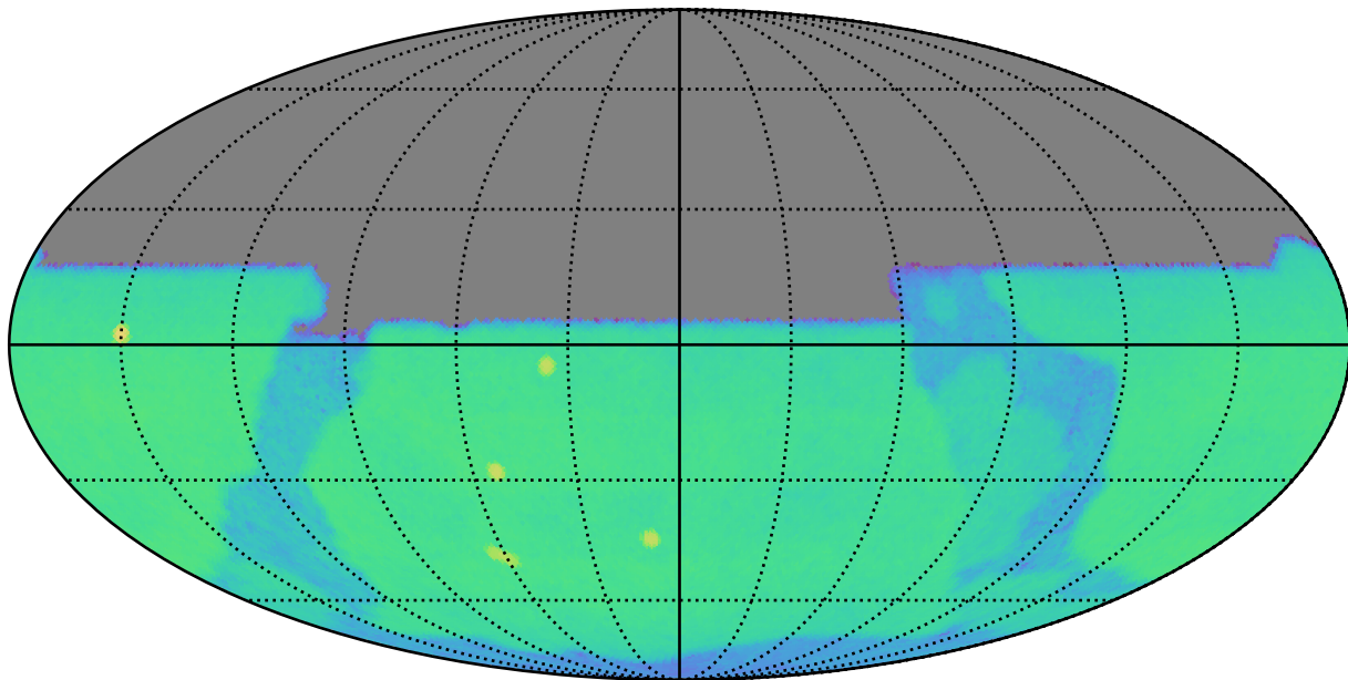
too_5_4v3.4_10yrs u: CoaddM5
