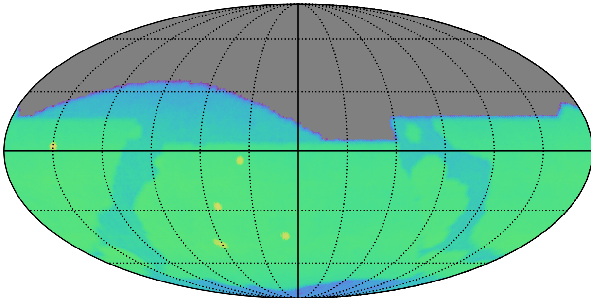
too_5_4v3.4_10yrs r: CoaddM5
