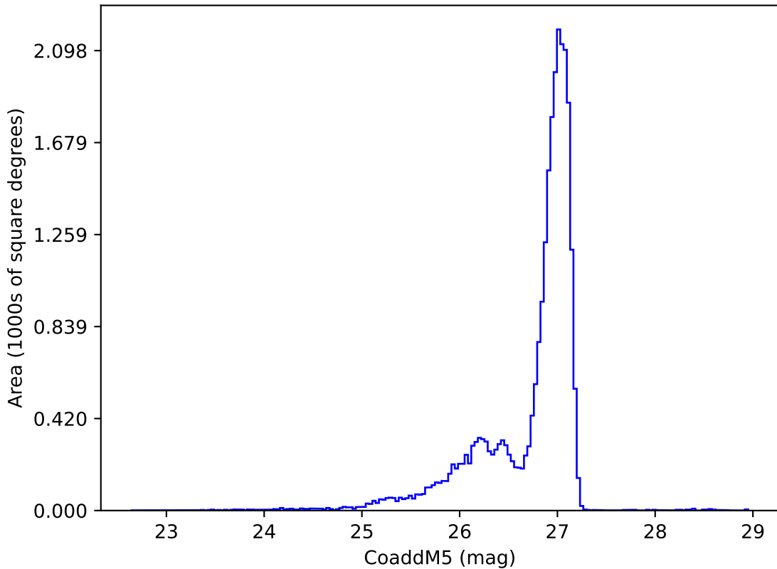
too_5_4v3.4_10yrs r: CoaddM5
