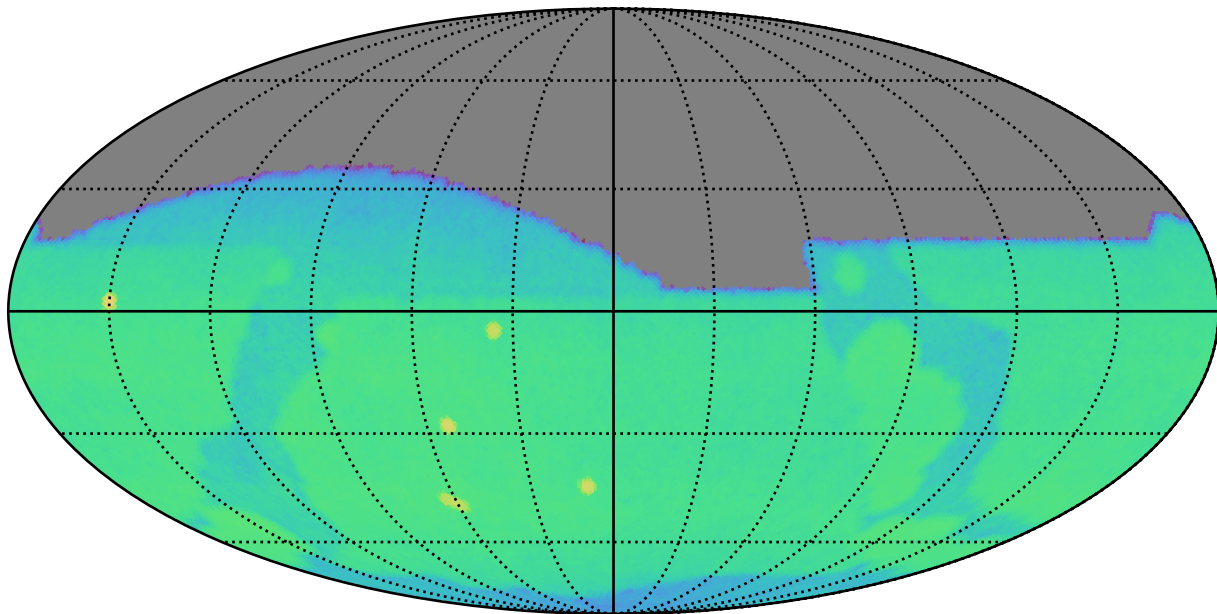
too_5_4v3.4_10yrs g: CoaddM5
