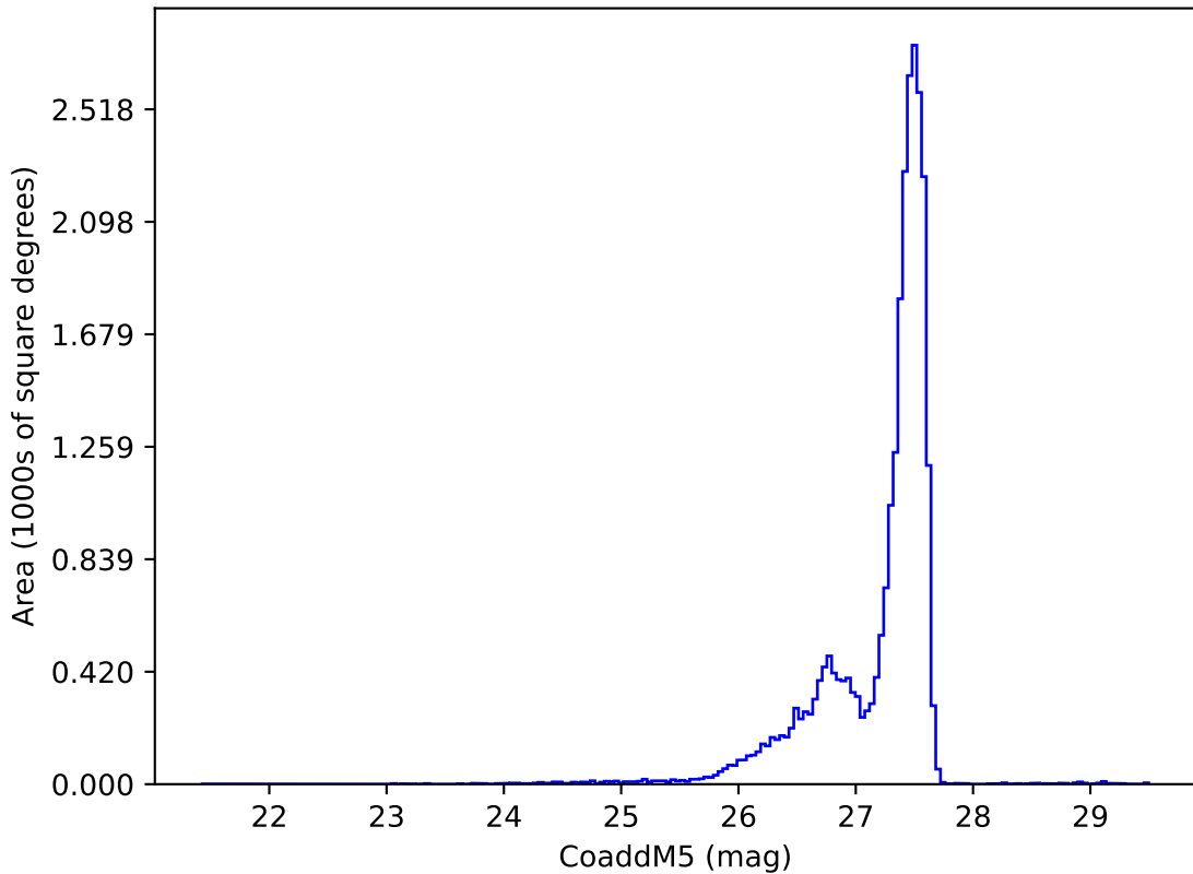
too_5_4v3.4_10yrs : CoaddM5
