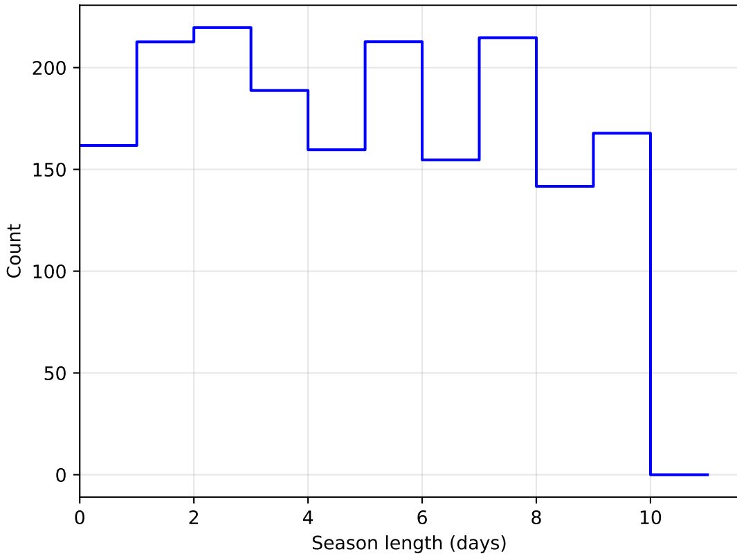
too_5_4v3.4_10yrs DD:WFD all bands: SeasonLength
