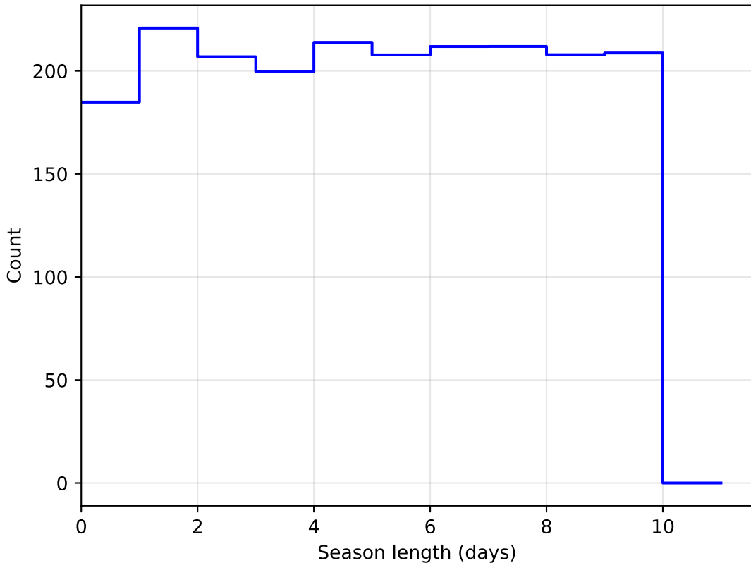
too_5_4v3.4_10yrs DD:ELAISS1 all bands: SeasonLength
