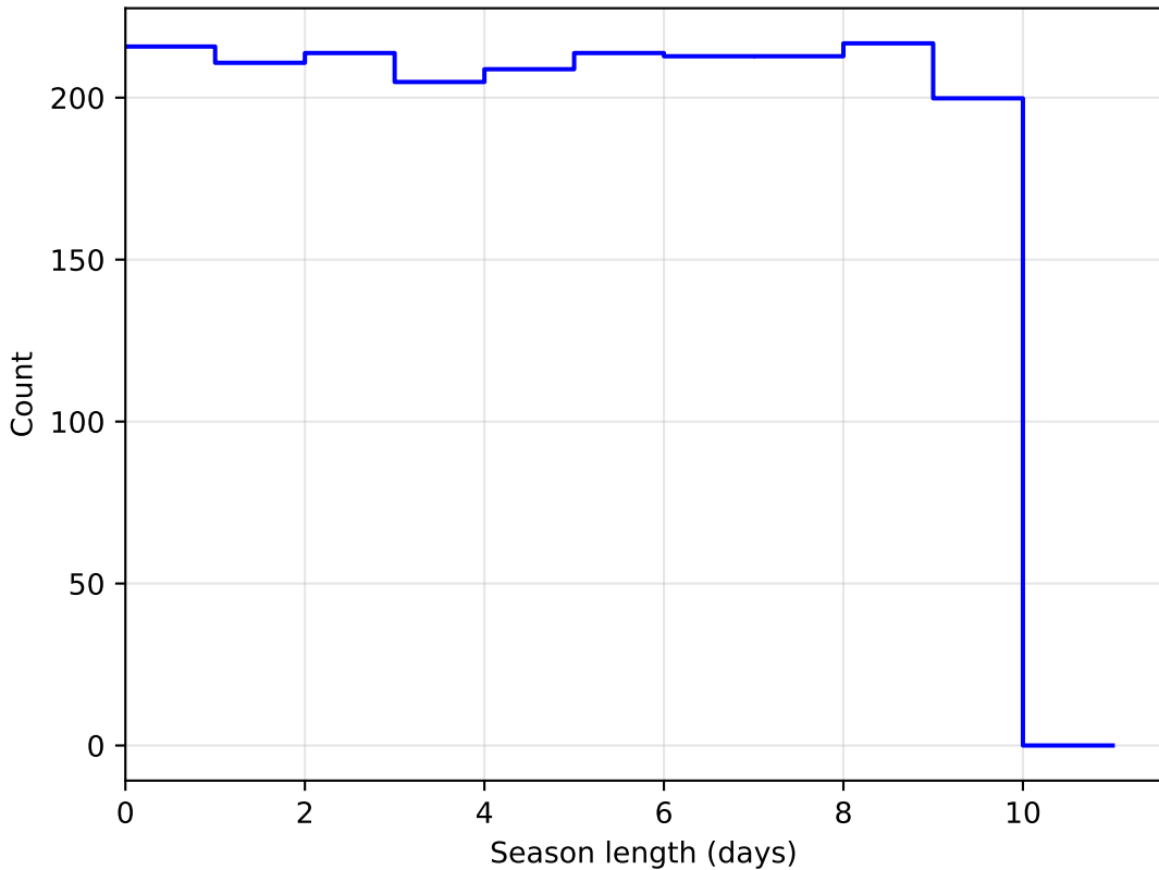
too_5_4v3.4_10yrs DD:ECDFS all bands: SeasonLength
