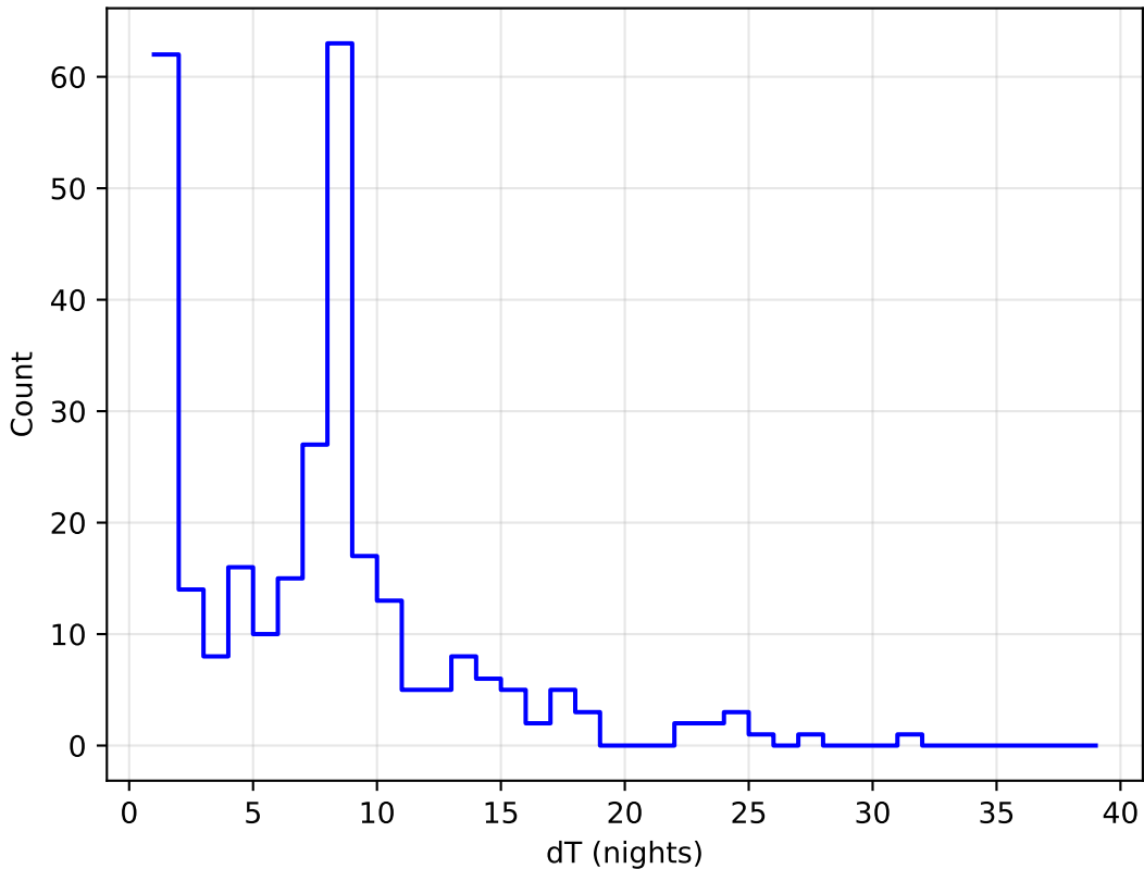
too_5_4v3.4_10yrs all bands: DD:XMM_LSS Delta Nights Histogram
