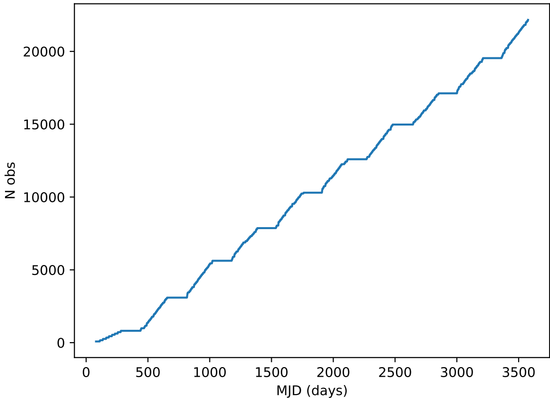
too_5_4v3.4_10yrs all bands: DD:XMM_LSS Cumulative NVisits
