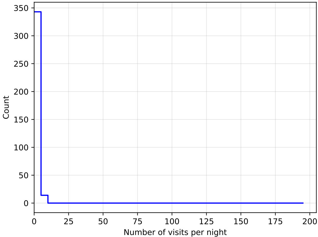
too_5_4v3.4_10yrs all bands: DD:WFD NVisitsPerNight
