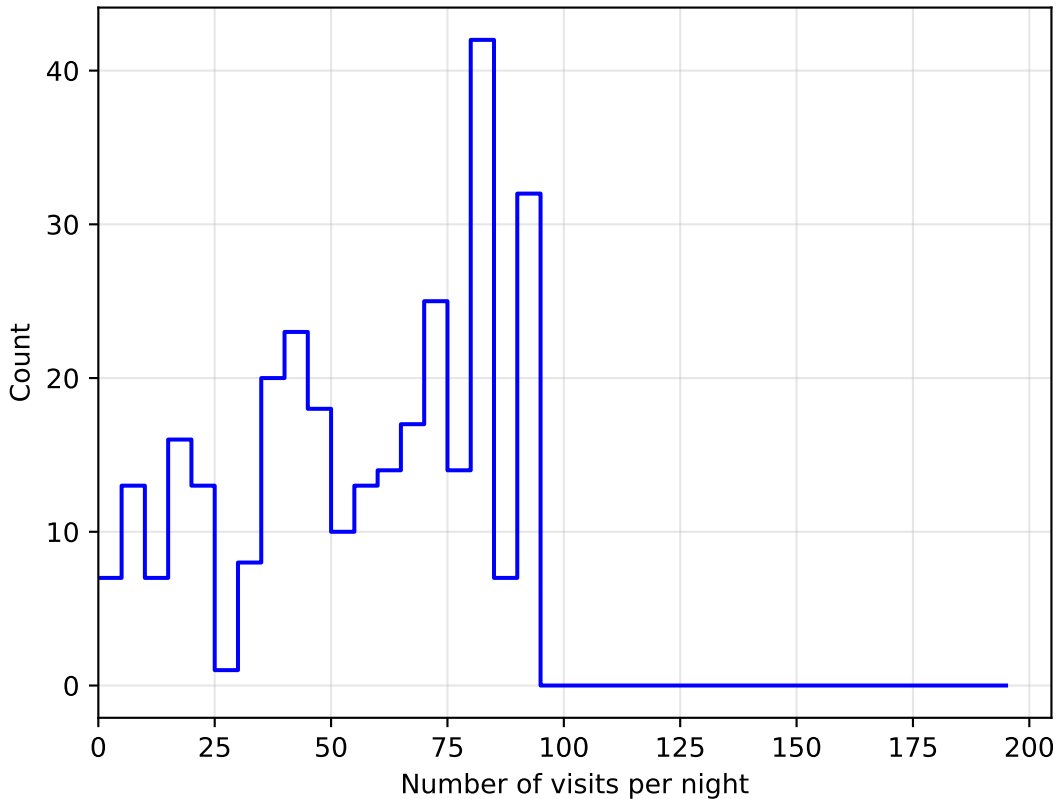
too_5_4v3.4_10yrs all bands: DD:EDFS NVisitsPerNight
