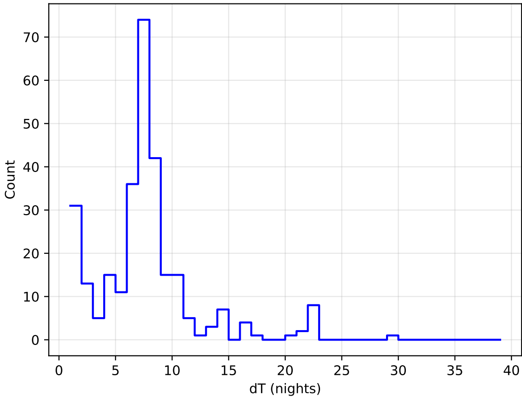
too_5_4v3.4_10yrs all bands: DD:EDFS Delta Nights Histogram
