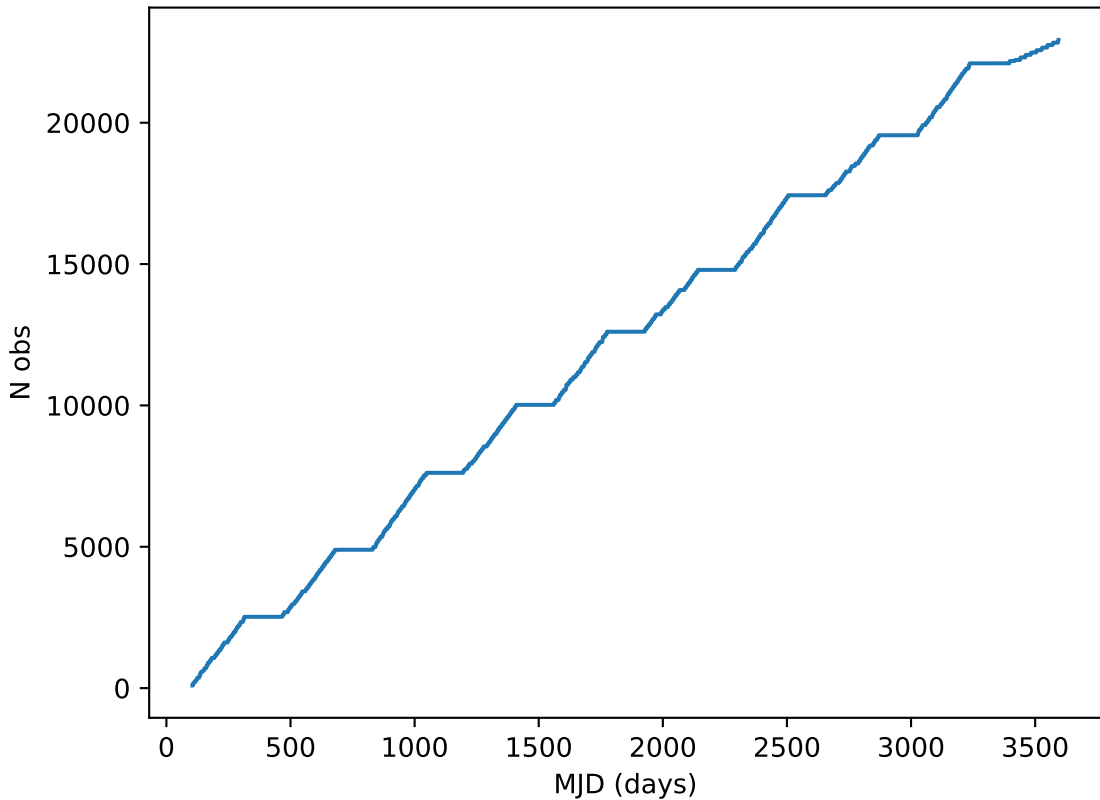
too_5_4v3.4_10yrs all bands: DD:EDFS Cumulative NVisits
