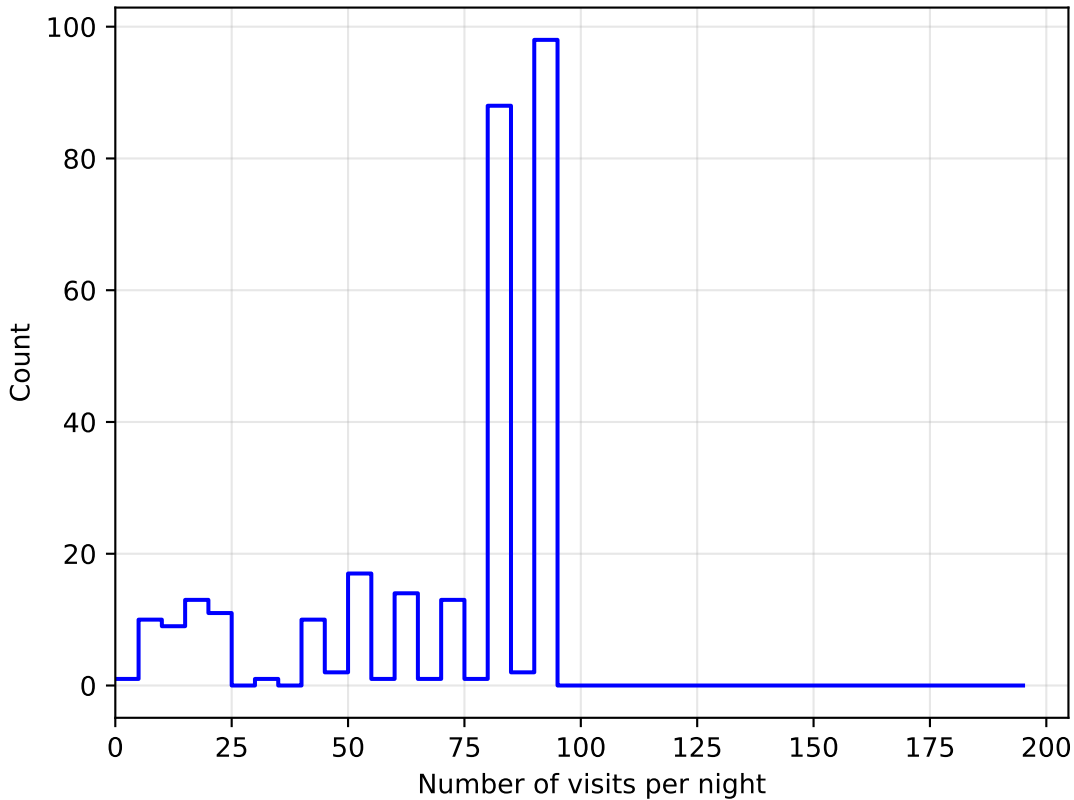
too_5_4v3.4_10yrs all bands: DD:ECDFS NVisitsPerNight
