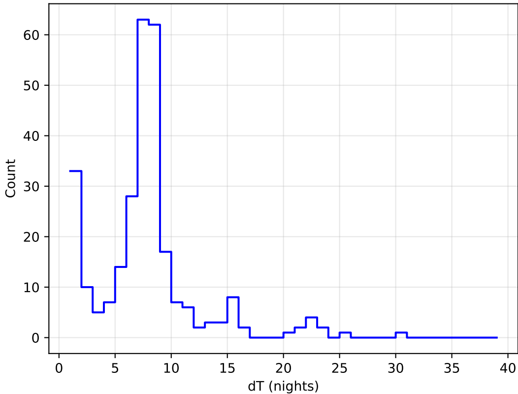
too_5_4v3.4_10yrs all bands: DD:ECDFS Delta Nights Histogram
