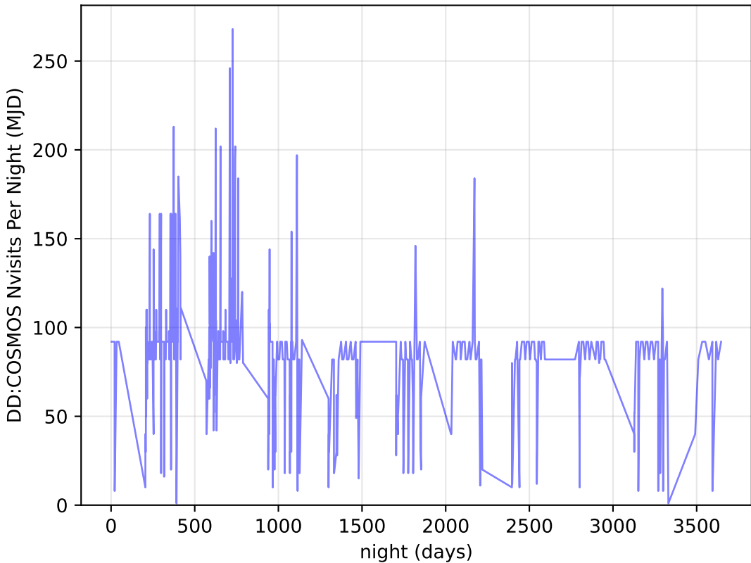
too_5_4v3.4_10yrs all bands: DD: COSMOS Nvisits Per Night
