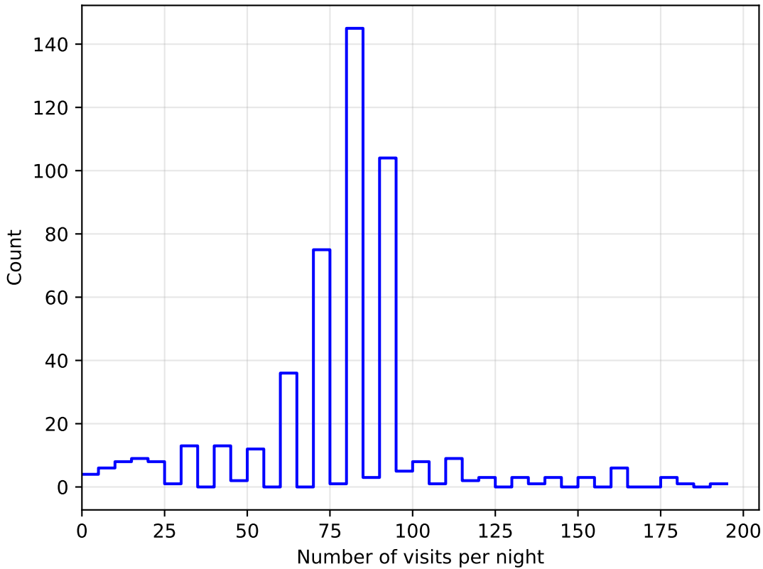
too_5_4v3.4_10yrs all bands: DD:COSMOS NVisitsPerNight
