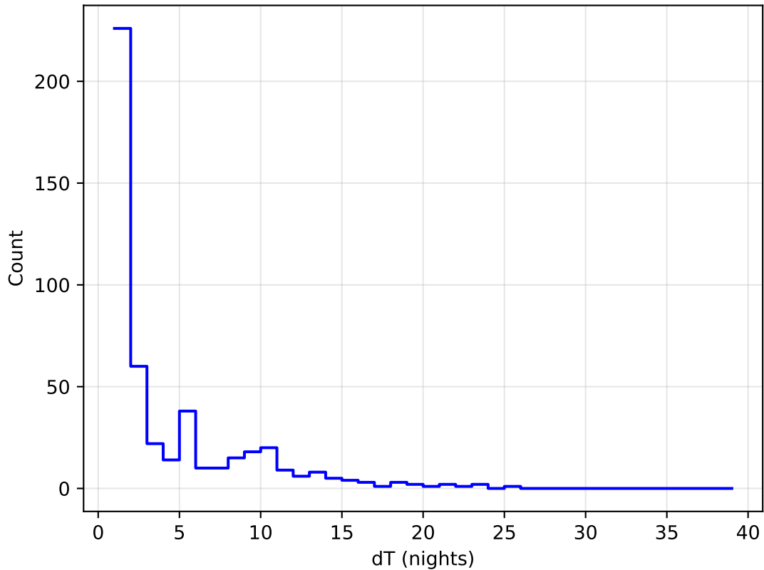
too_5_4v3.4_10yrs all bands: DD:COSMOS Delta Nights Histogram
