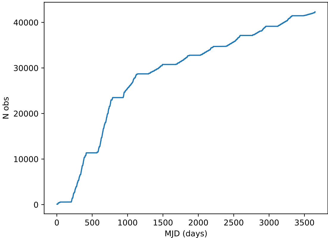
too_5_4v3.4_10yrs all bands: DD: COSMOS Cumulative NVisits
