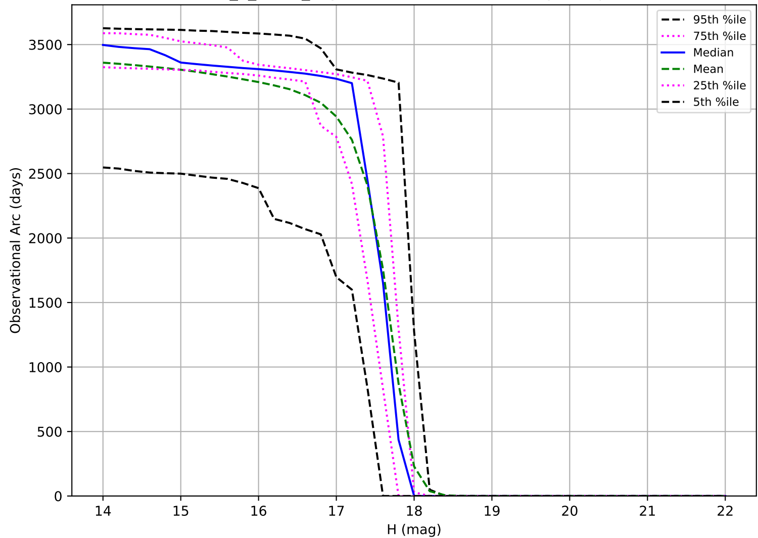
too_5_1v3.4_10yrs: Observational Arc Length Trojan
