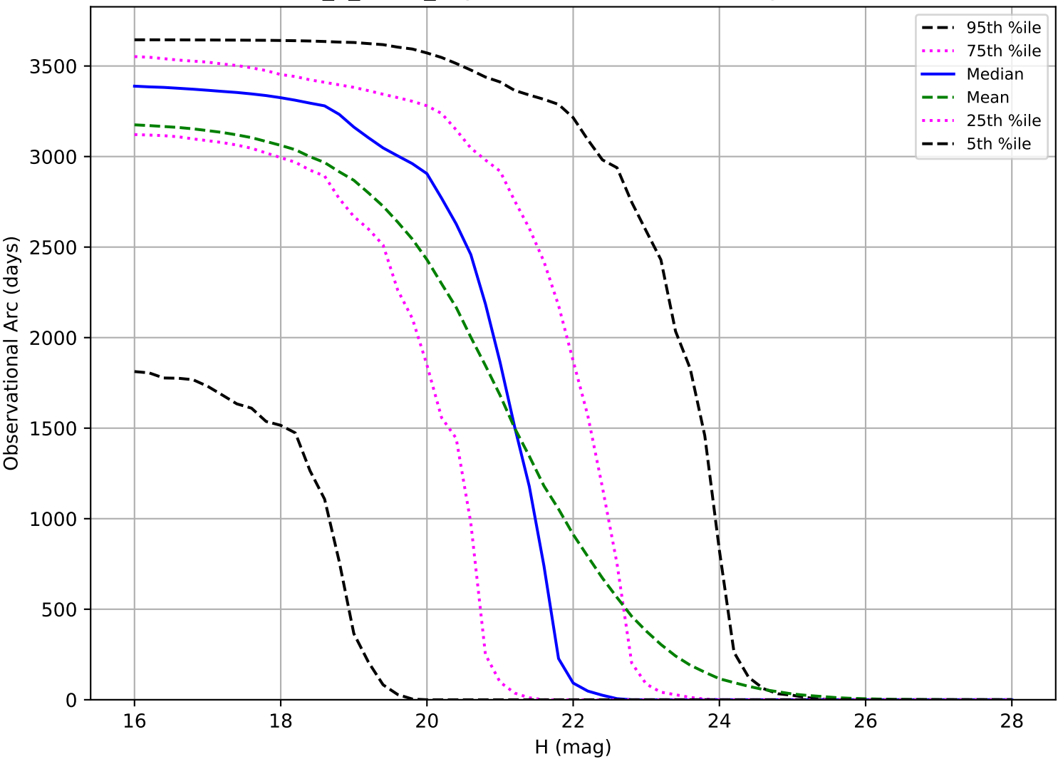
too_5_1v3.4_10yrs: Observational Arc Length NEO
