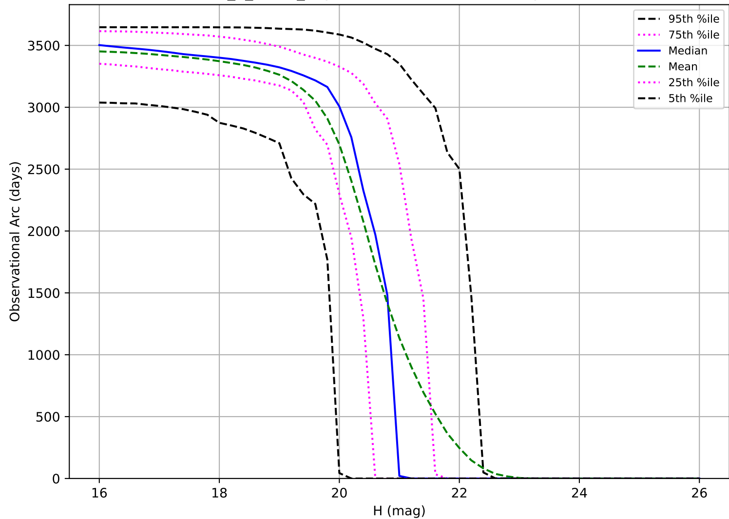
too_5_1v3.4_10yrs: Observational Arc Length MBA
