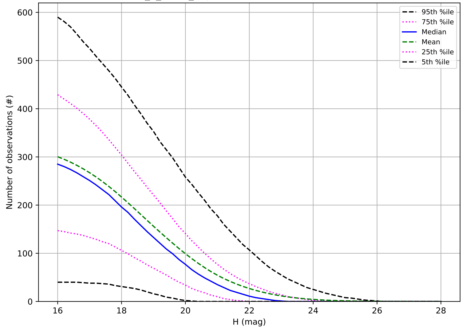
too_5_1v3.4_10yrs: Number of observations PHA
