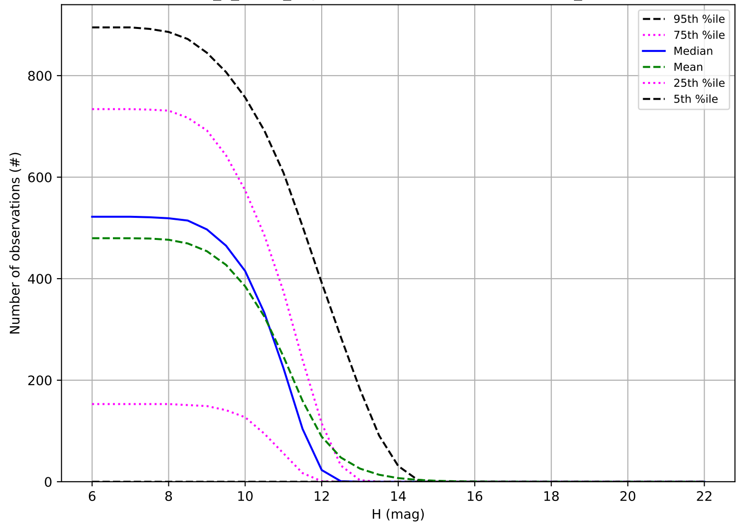
too_5_1v3.4_10yrs: Number of observations OCC_r20
