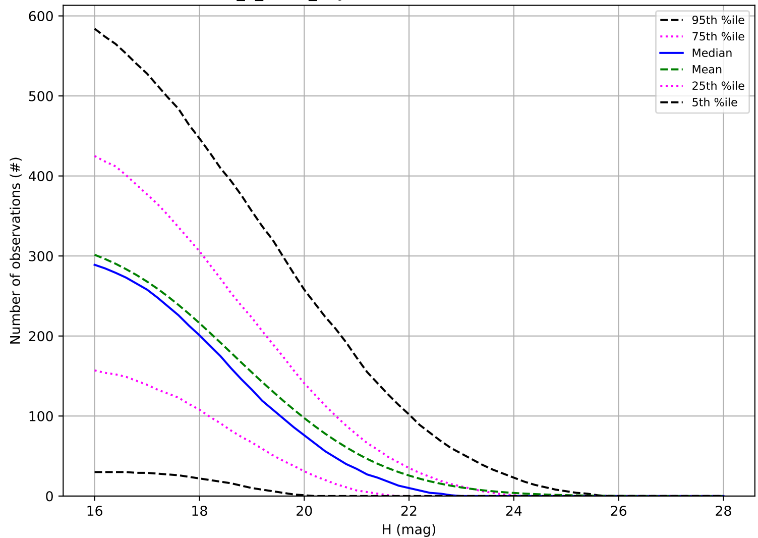
too_5_1v3.4_10yrs: Number of observations NEO
