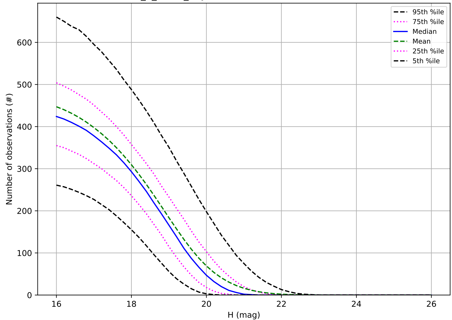
too_5_1v3.4_10yrs: Number of observations MBA
