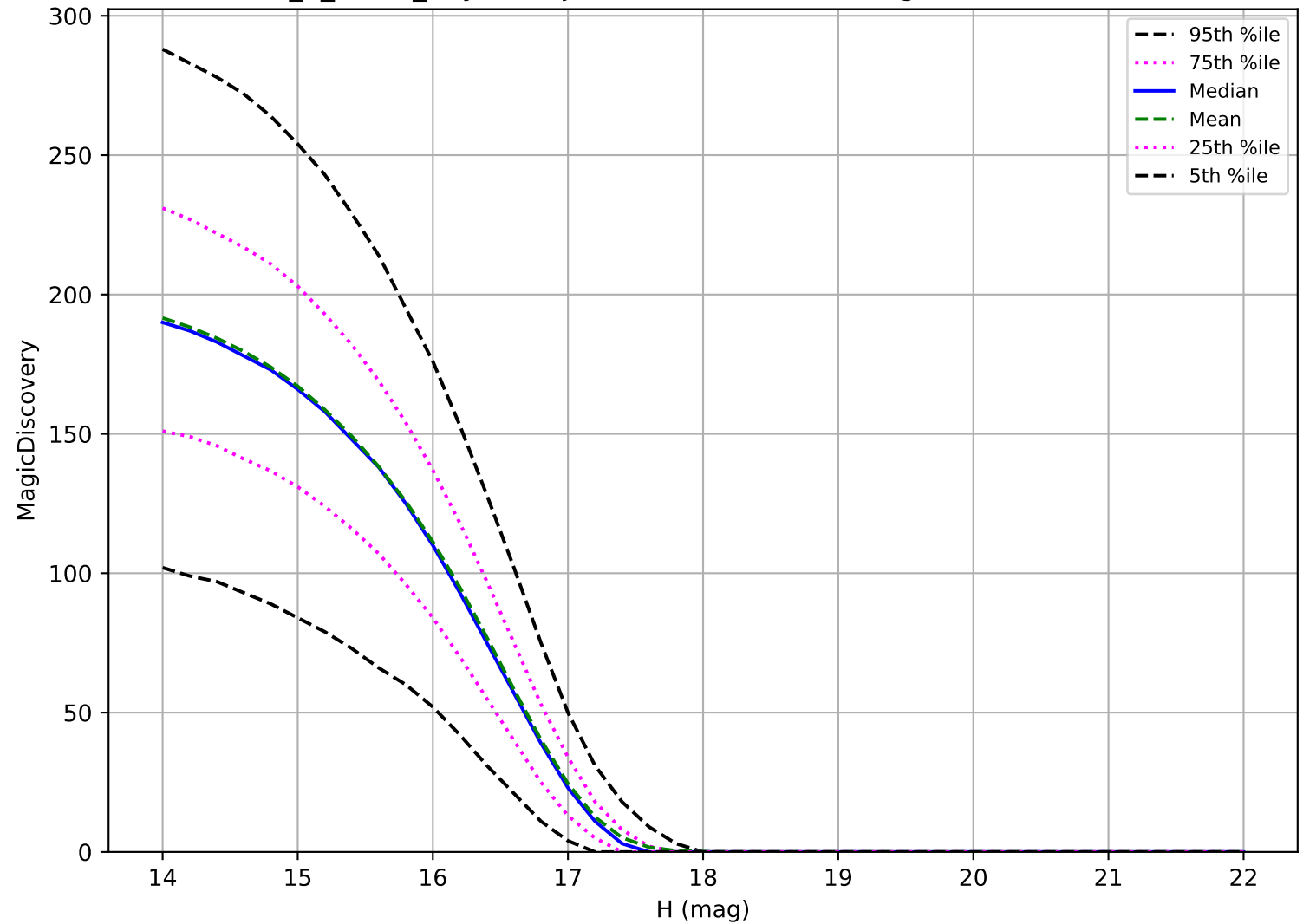
too_5_1v3.4_10yrs: Trojan 6 detections in 60 nights detection loss
