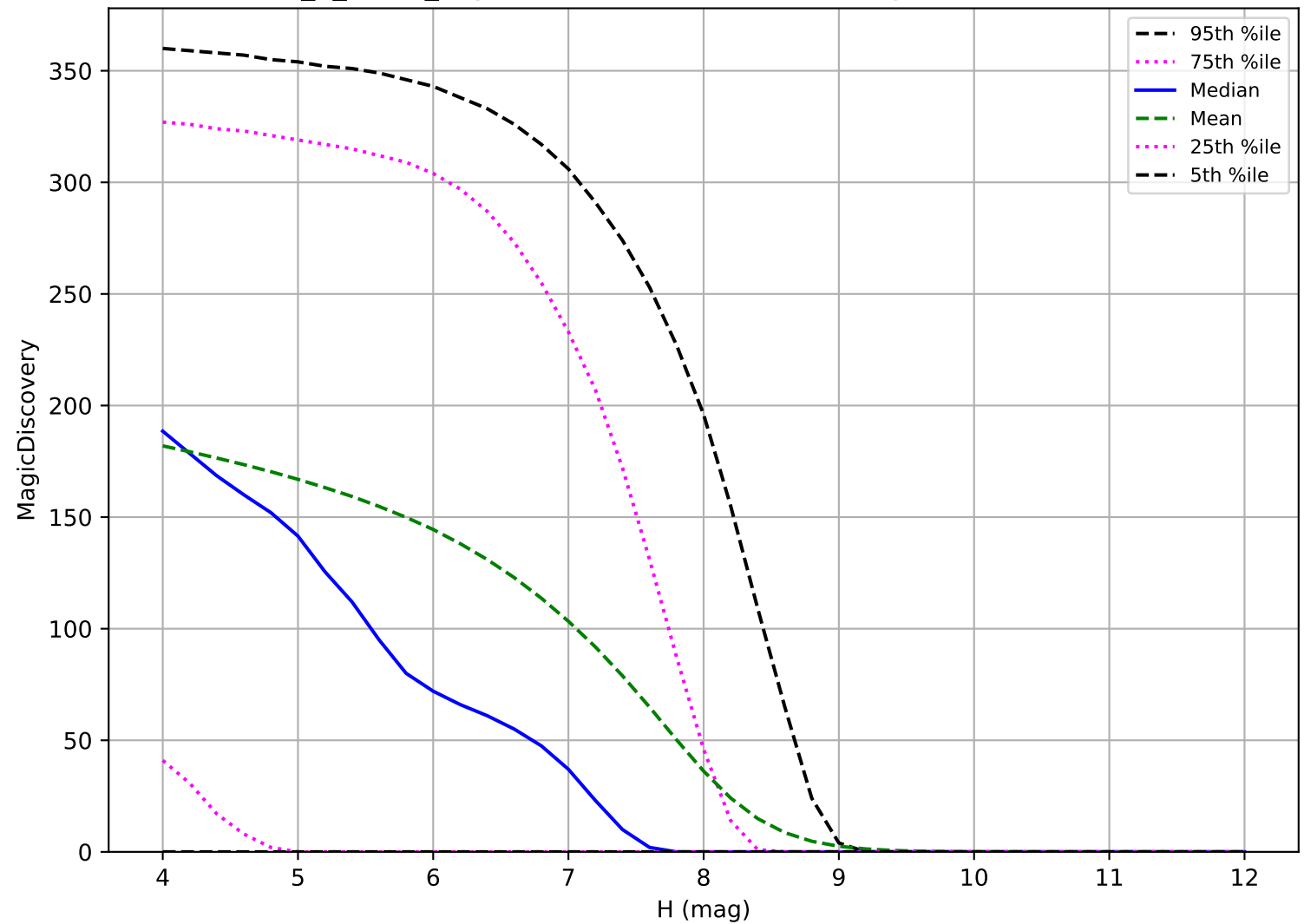
too_5_1v3.4_10yrs: TNO 6 detections in 60 nights detection loss
