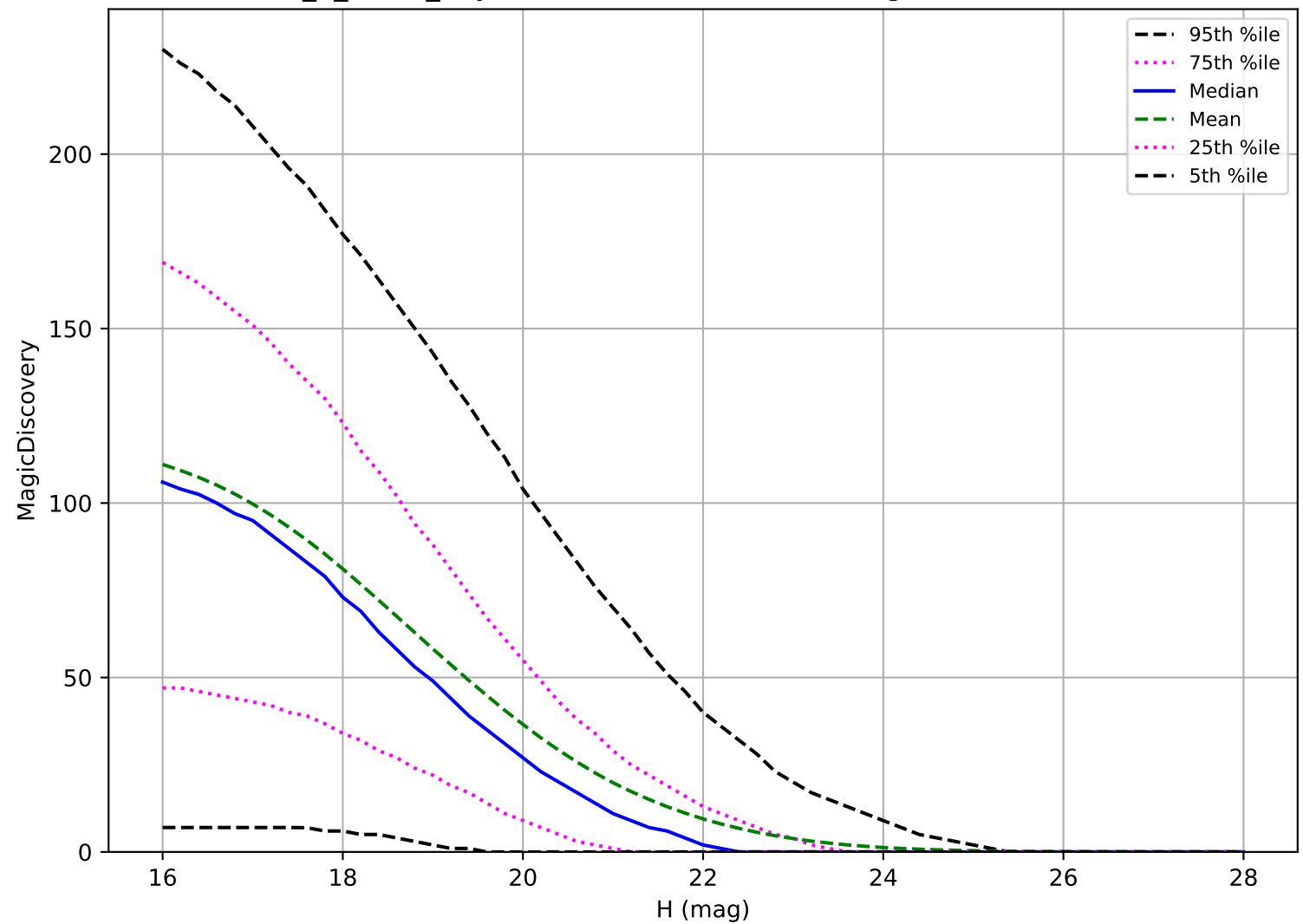
too_5_1v3.4_10yrs: PHA 6 detections in 60 nights detection loss
