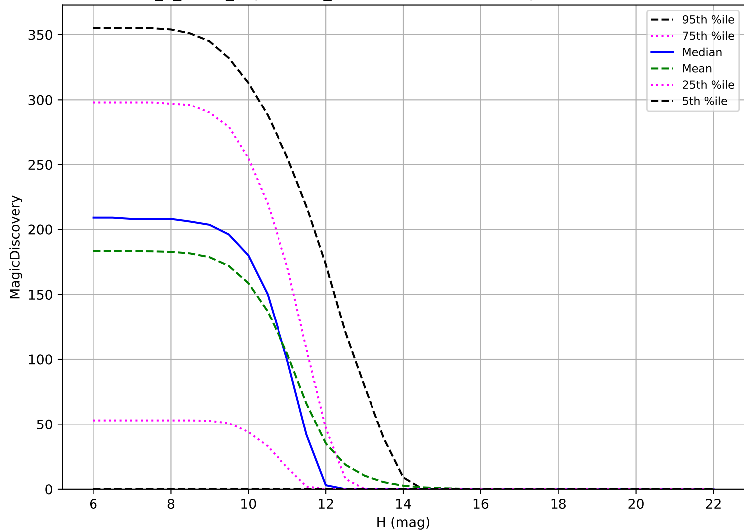
too_5_1v3.4_10yrs: OCC_r20 6 detections in 60 nights detection loss
