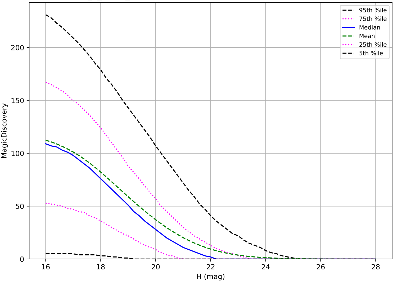
too_5_1v3.4_10yrs: NEO 6 detections in 60 nights detection loss
