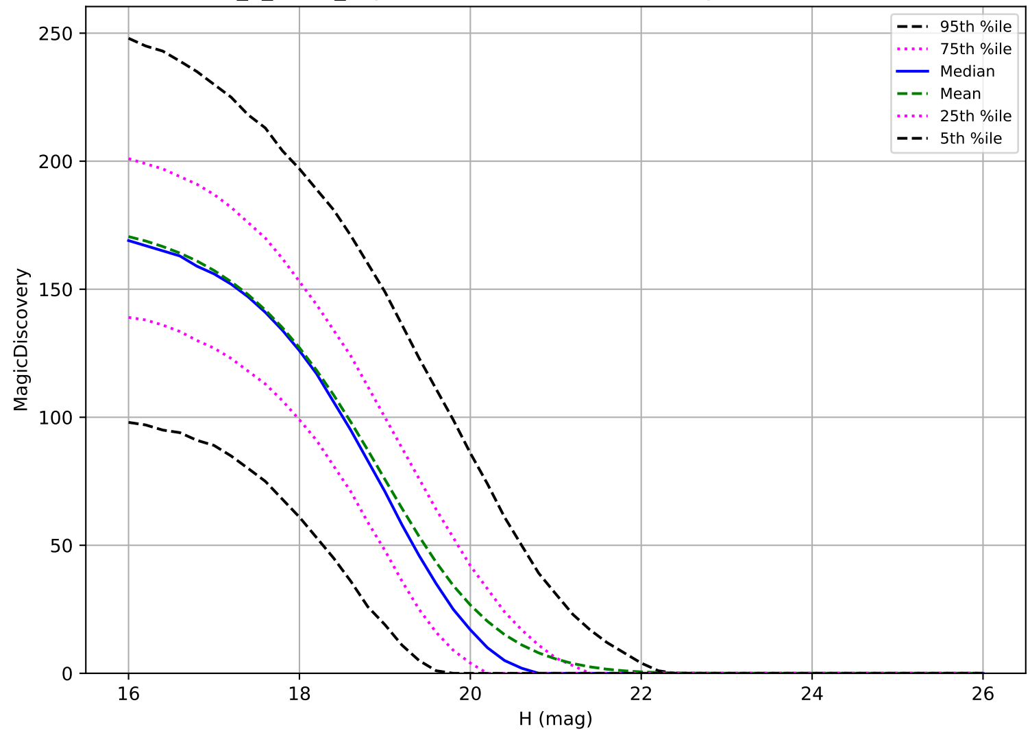
too_5_1v3.4_10yrs: MBA 6 detections in 60 nights detection loss
