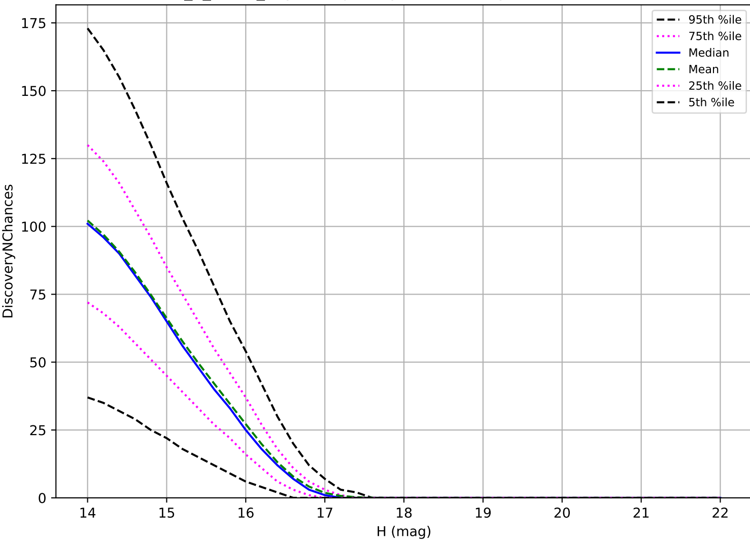
too_5_1v3.4_10yrs: Trojan 3 pairs in 15 nights detection loss
