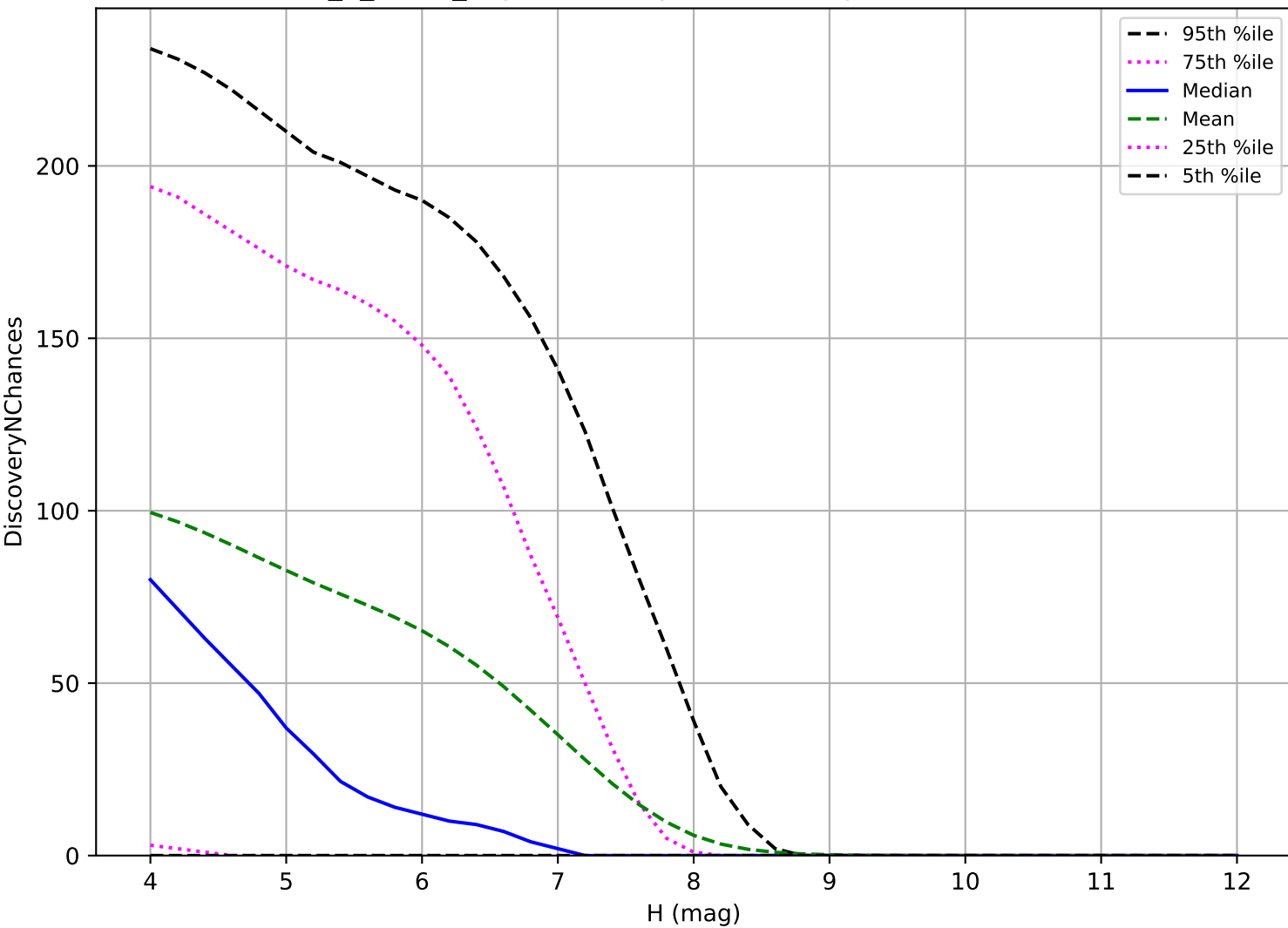
too_5_1v3.4_10yrs: TNO 3 pairs in 15 nights detection loss
