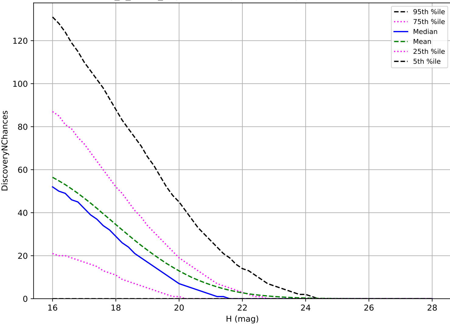
too_5_1v3.4_10yrs: NEO 3 pairs in 15 nights detection loss
