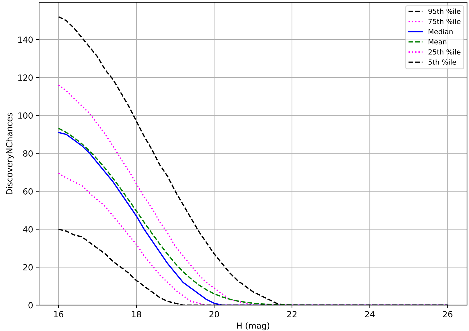
too_5_1v3.4_10yrs: MBA 3 pairs in 15 nights detection loss
