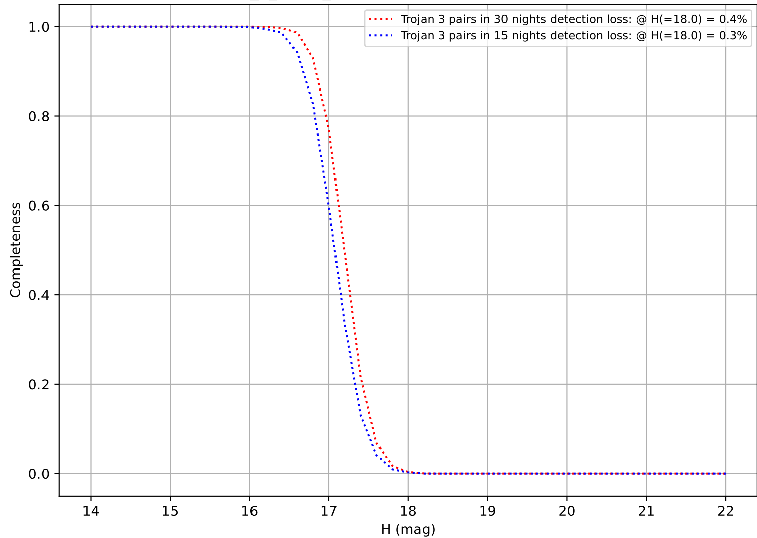
too_5_1v3.4_10yrs: DifferentialCompleteness
