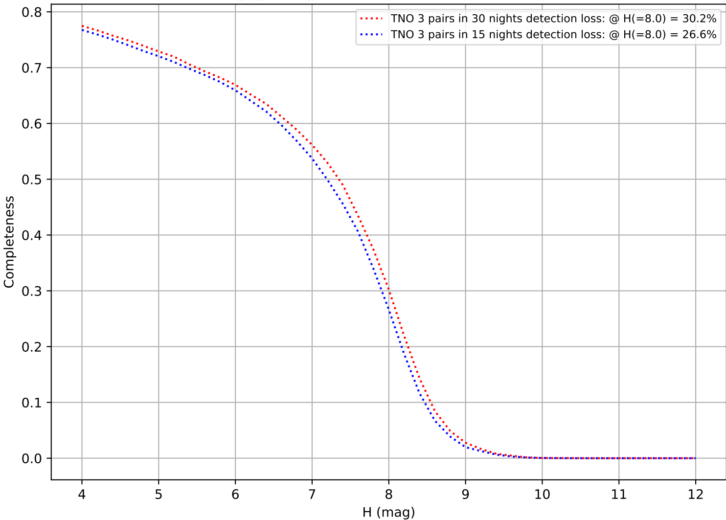
too_5_1v3.4_10yrs: DifferentialCompleteness
