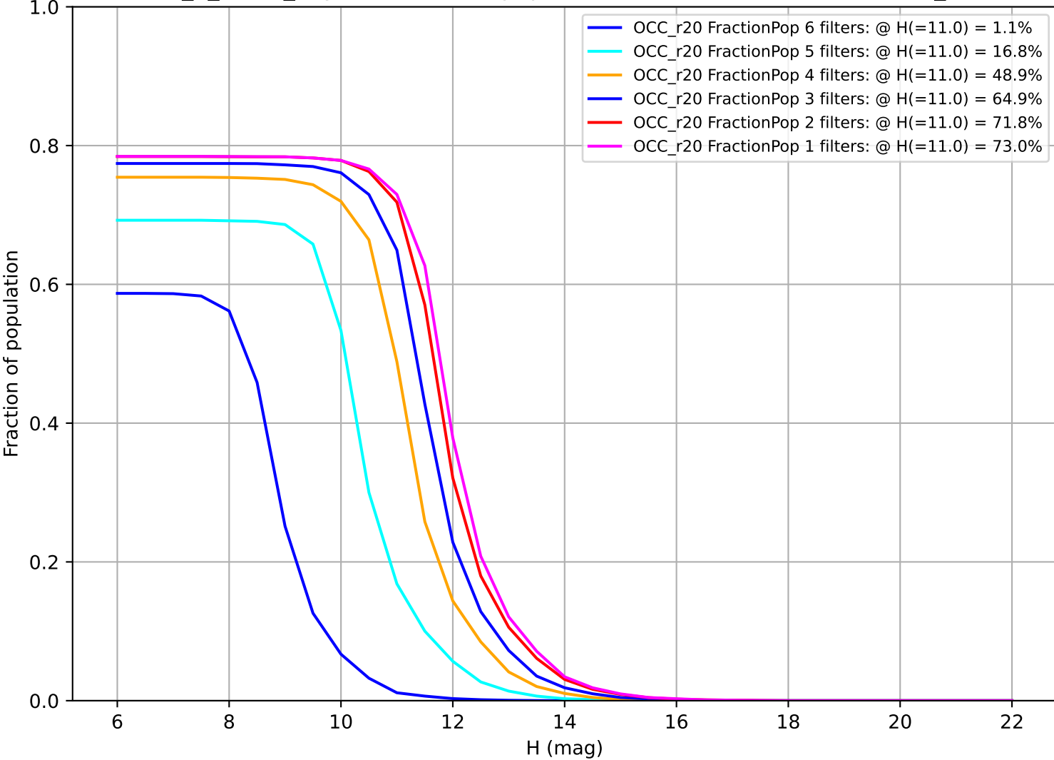
too_5_1v3.4_10yrs: Fraction of population with colors in X filters OCC_r20
