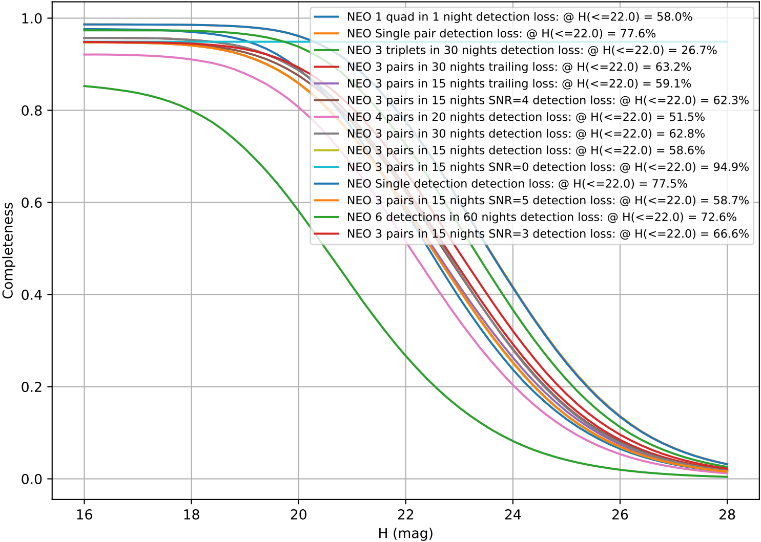
too_5_1v3.4_10yrs: CumulativeCompleteness
