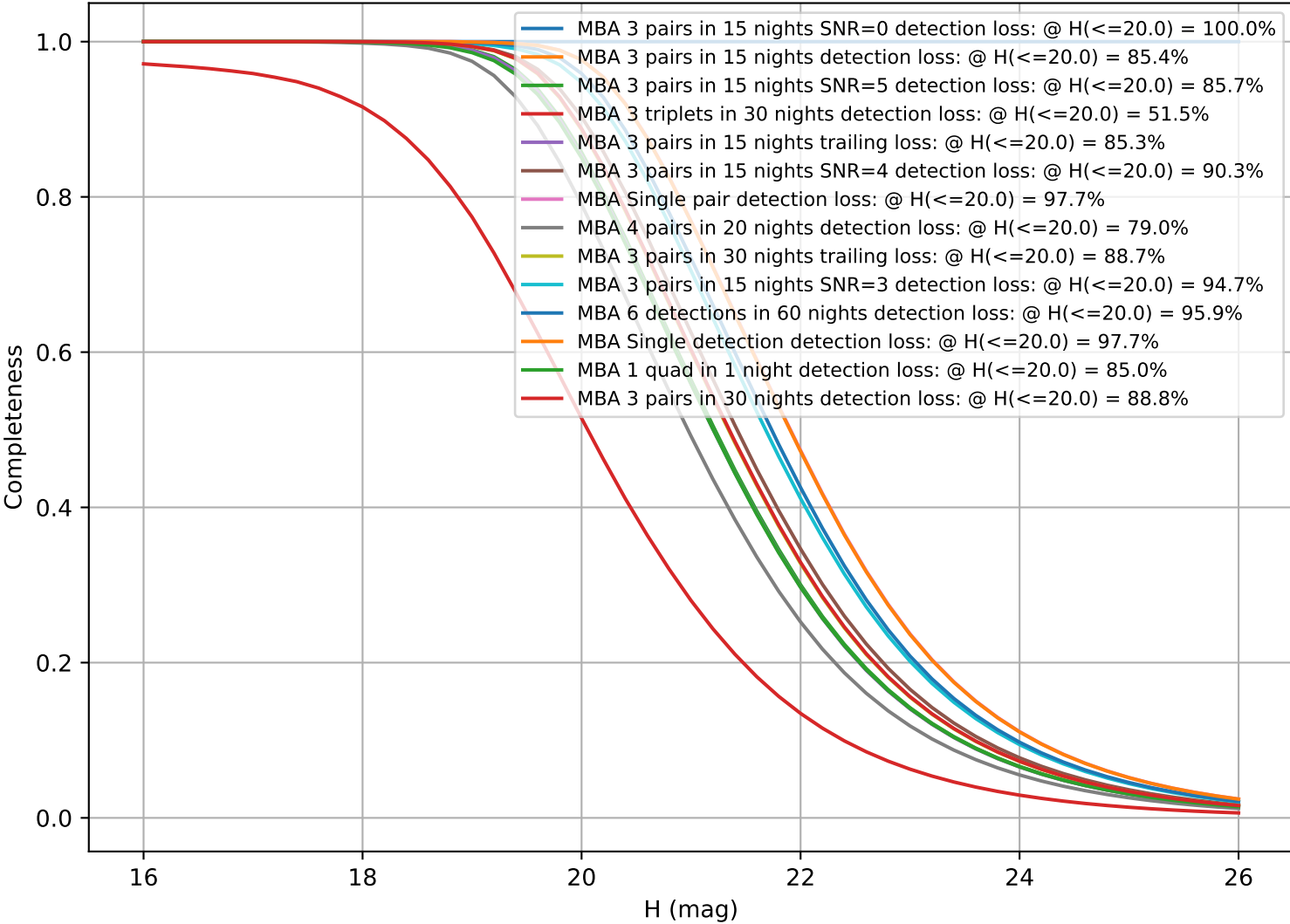
too_5_1v3.4_10yrs: CumulativeCompleteness
