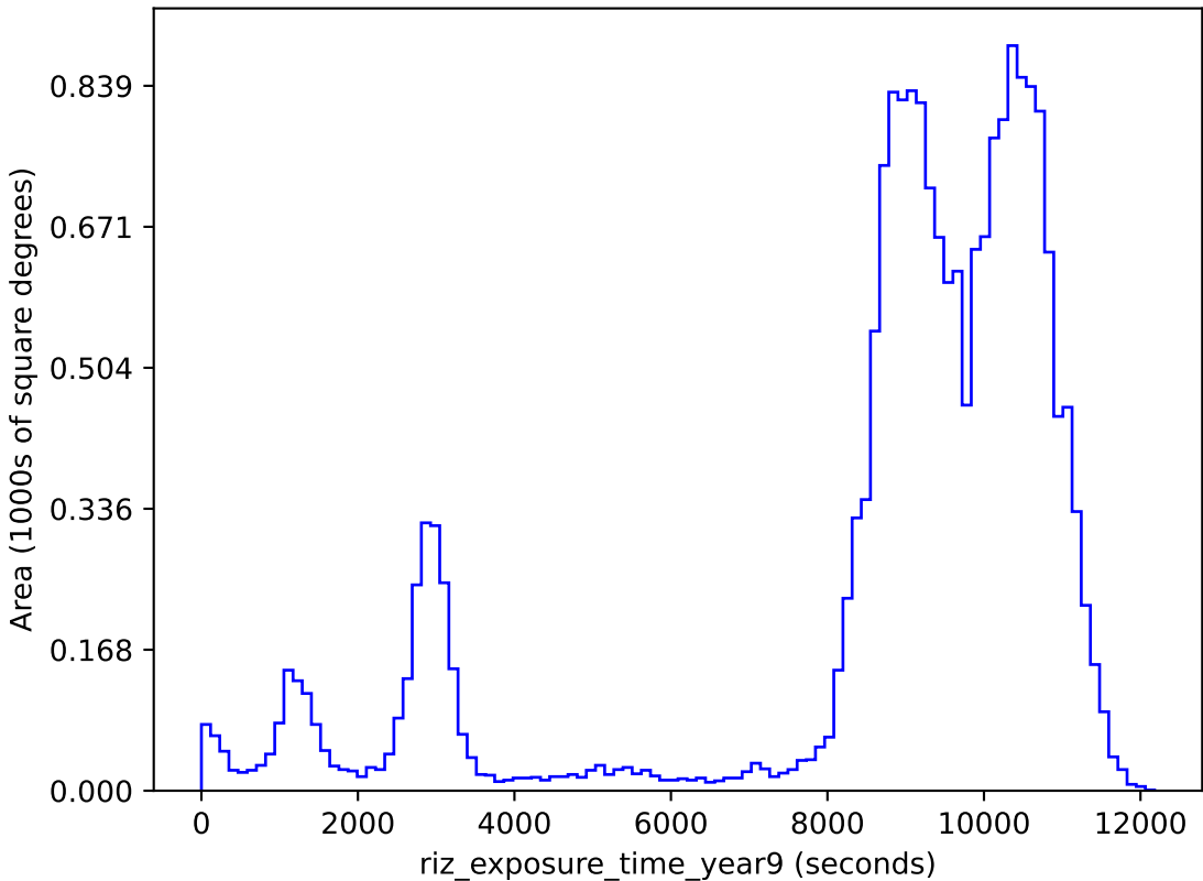
too_5_1v3.4_10yrs gri band non-DD: riz_exposure_time_year9
