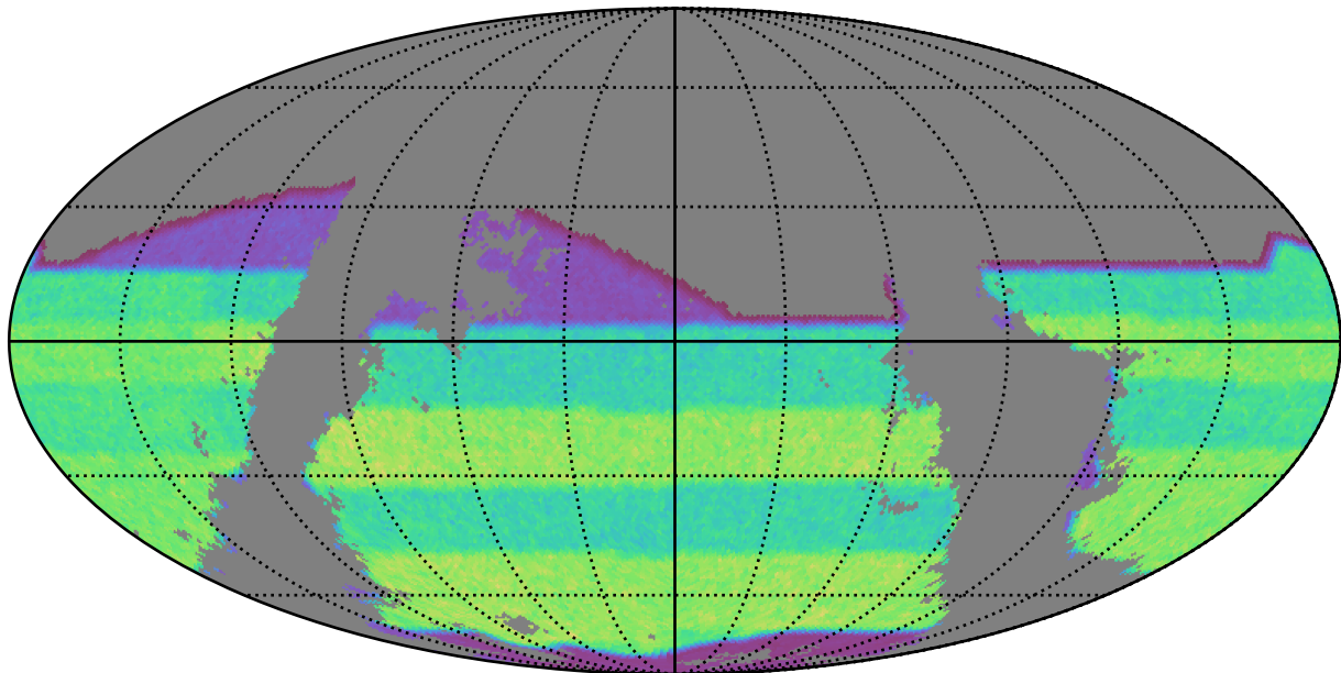
too_5_1v3.4_10yrs gri band non-DD: riz_exposure_time_year5
