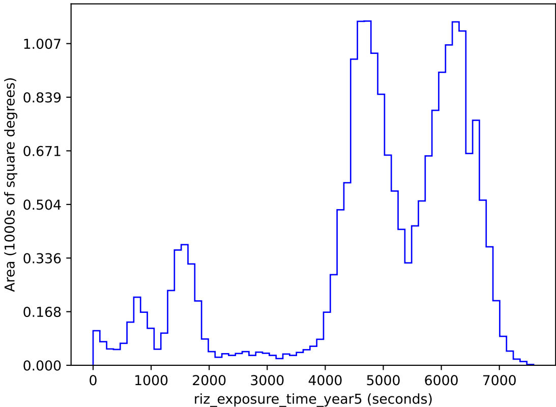
too_5_1v3.4_10yrs gri band non-DD: riz_exposure_time_year5
